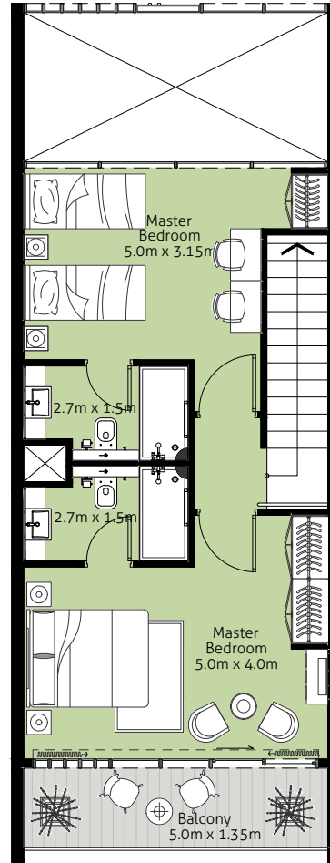
First Floor
