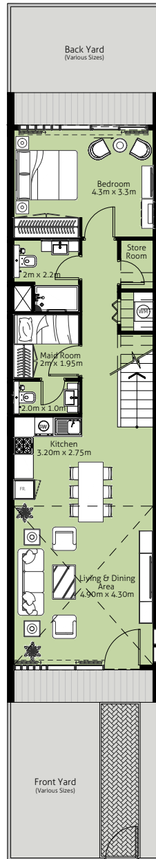
Ground Floor
